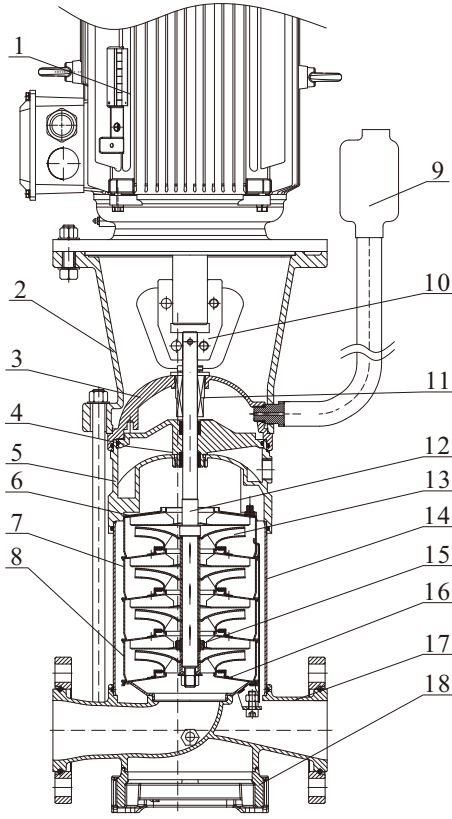
结构图ASF8,10,12,15,16,20
